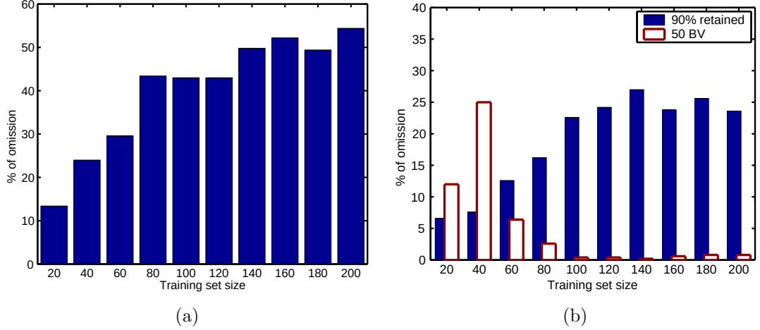
Figure 3.4: Omission rates caused by the simplified \mathcal{BV} score, eq. (3.26) when applied to the Friedman #1 data. Subfigure (a) shows the omission at the end of a sequence of full training, while in subfigure (b) we plotted the errors made when the \mathcal{BV} set size was set to 90% of the training set (full bars) and to 50, irrespective of the size of the training set (empty bars). Note that the range of the Y-axis differs in the two sub-plots.
